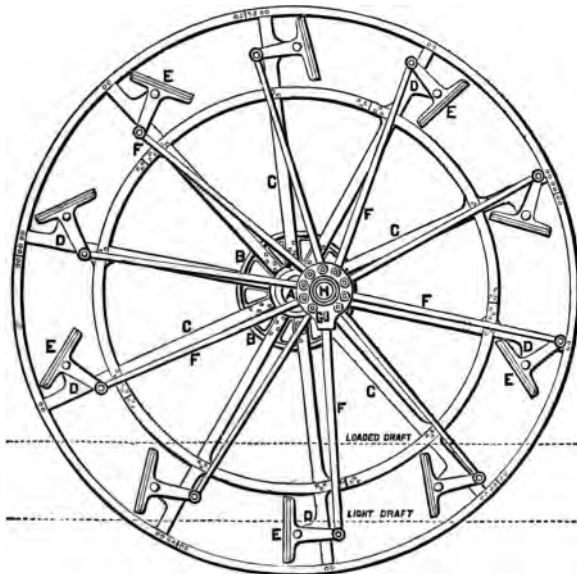
FIG. 87.—The Feathering Paddle-Wheel.
